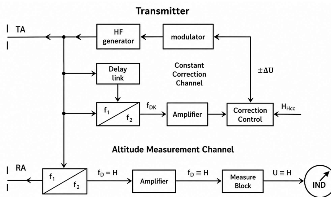
Fig. 36 Correction of the measurement result by the radio altimeter constant
